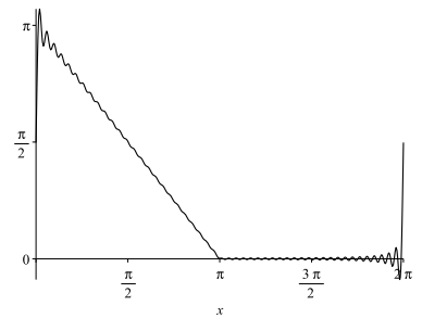
Figure 2.8: A plot of first terms of the Fourier series of f(x) in Problem 2.9e.
