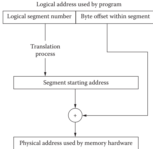
Figure 2.19 Address translation in a system with demand-segmented virtual memory.
