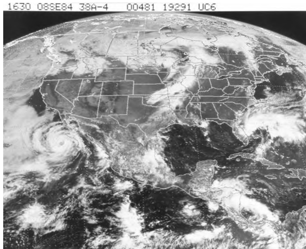
GOES image of North America (Multispectral Geostationary Operational Environment Satellite)
