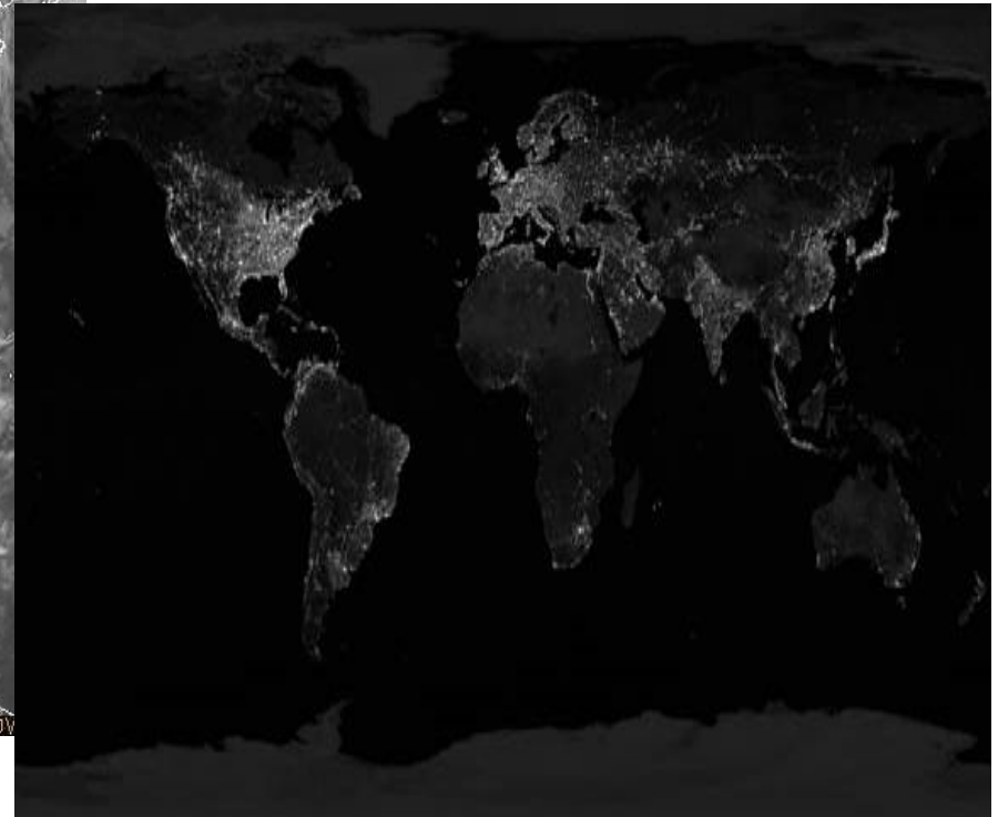
Infrared satellite imagery in the near infrared band
