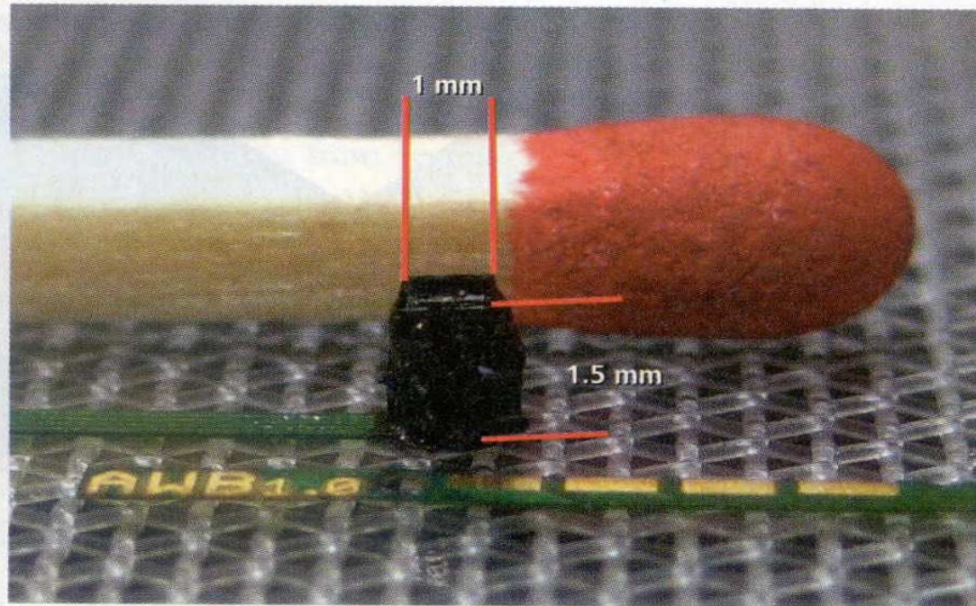
FIGURE 1. In the development of Awaiba's NanEye miniature camera, individual lenses, sensors, and readout electronics are fabricated at the wafer level and then bonded to form a single camera.
