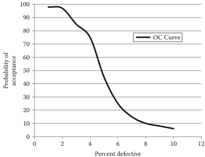
Figure 2.12 Operating characteristic curve for a particular sampling plan.
