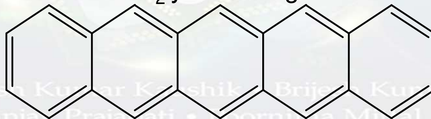
Pentacene
