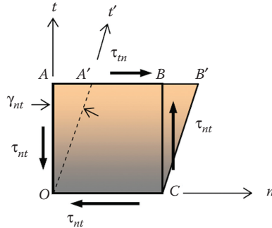
FIGURE 2.7 Definition of shearing strain \gamma_{nt} as being approximately equal to the tangent of the shearing angle \gamma_{nt} .
