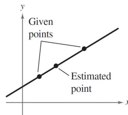
Linear interpolation
