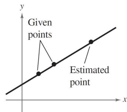
Linear extrapolation
