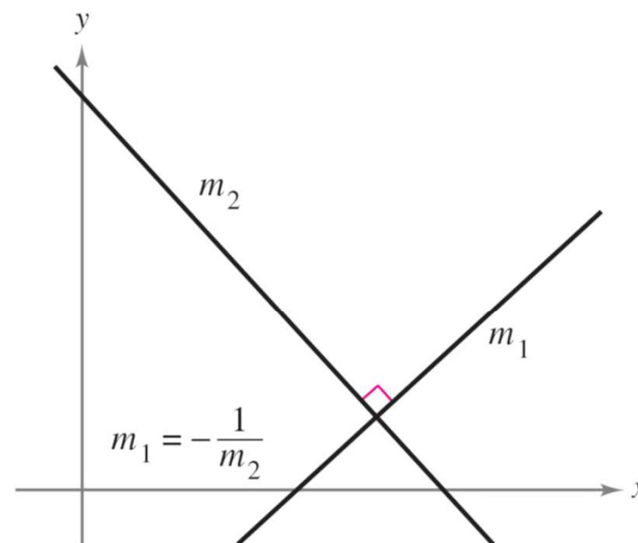
Perpendicular lines
