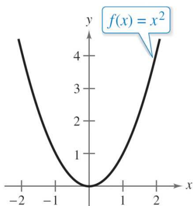
(e) Quadratic Function
