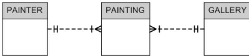
FIGURE P2.10b The UBA Relational Model
