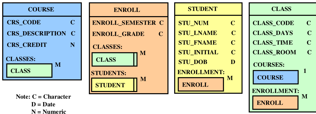
Figure P2.8b The UML Model for Tiny College
