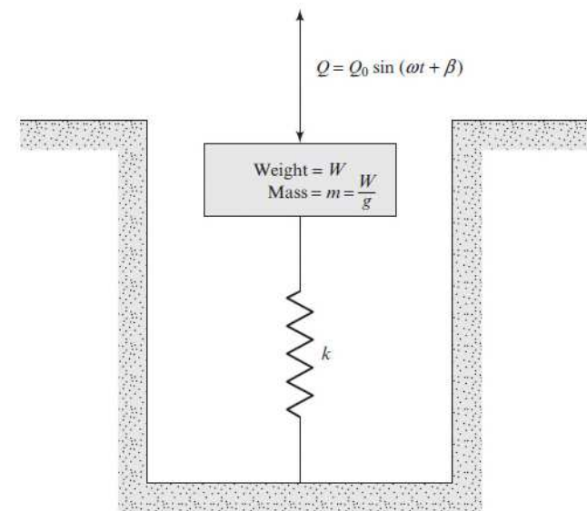
Figure 2.6 Forced vibration of mass-spring system title
