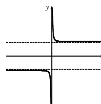
Two horizontal asymptotes
