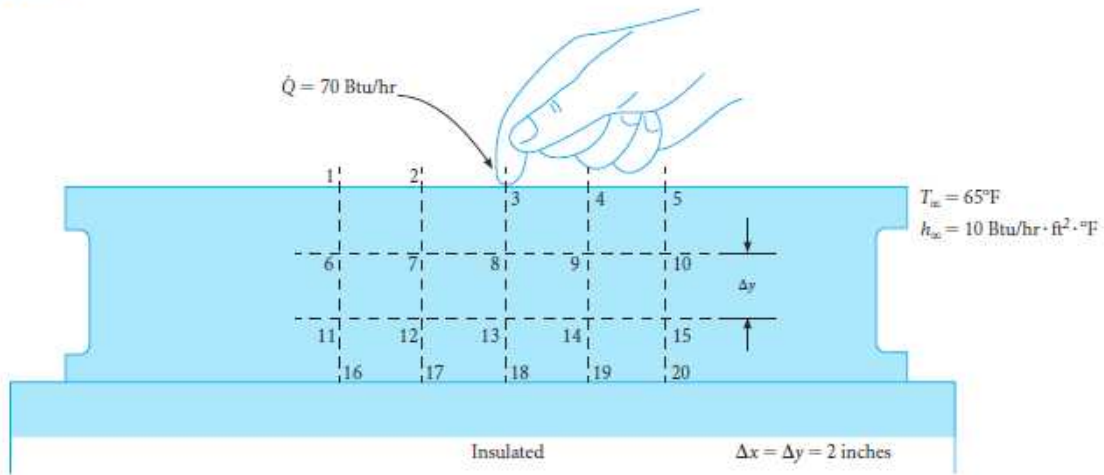
FIG 2-70 Surface plate.
