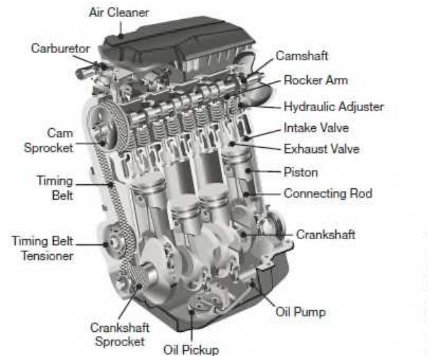
FIGURE 2.22 Rotating shaft work can be found in many devices, including a turbine and the crankshaft of a reciprocating engine.
