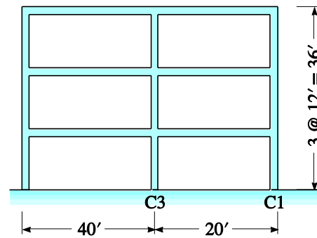
Building Section
