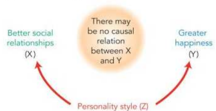
(c) Third-variable problem
