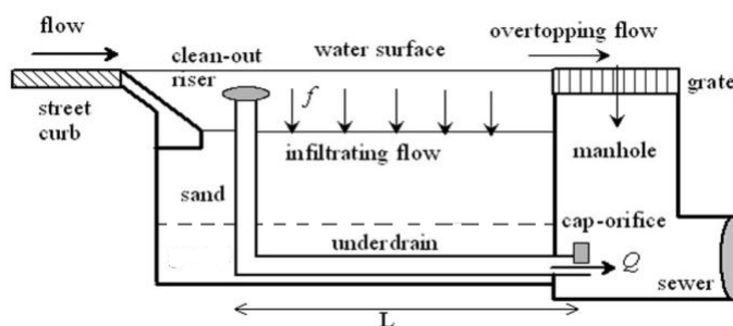
Construction of LID Rain Garden
