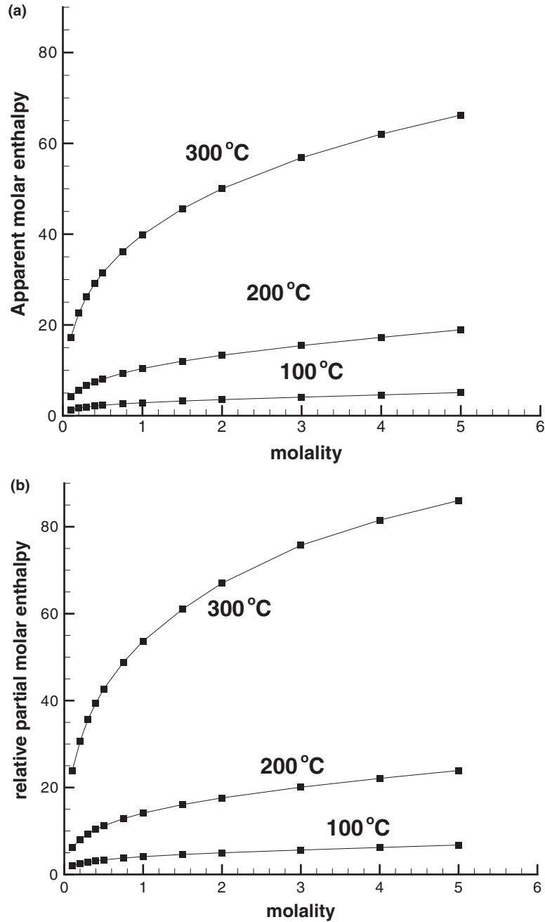
Figure 10.11 (a) The apparent relative molar enthalpy of NaCl ( \phi L_2 ), from the data in Figure 10.10. (b) The relative partial molar enthalpy ( \bar{L}_2 ) of NaCl from the data in Figure 10.10. Data from Busey et al. (1984).
