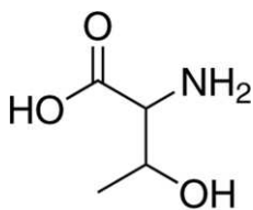
threonine
