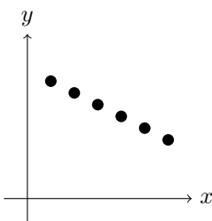
Figure 2.3: Scatterplot for situation 2
