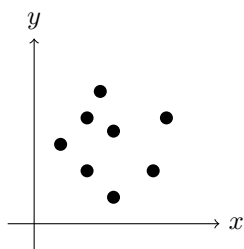
Figure 2.2: Scatterplot for situation 1
