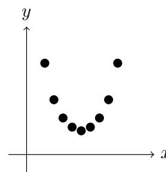
Figure 2.4: Scatterplot for situation 3
