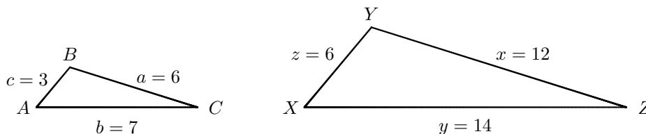
Figure 2.7: Two similar triangles
