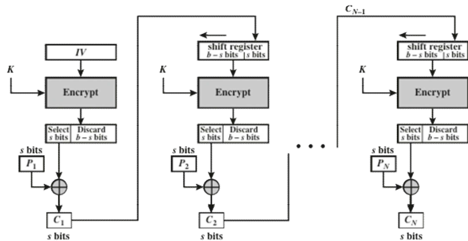
(a) Encryption
