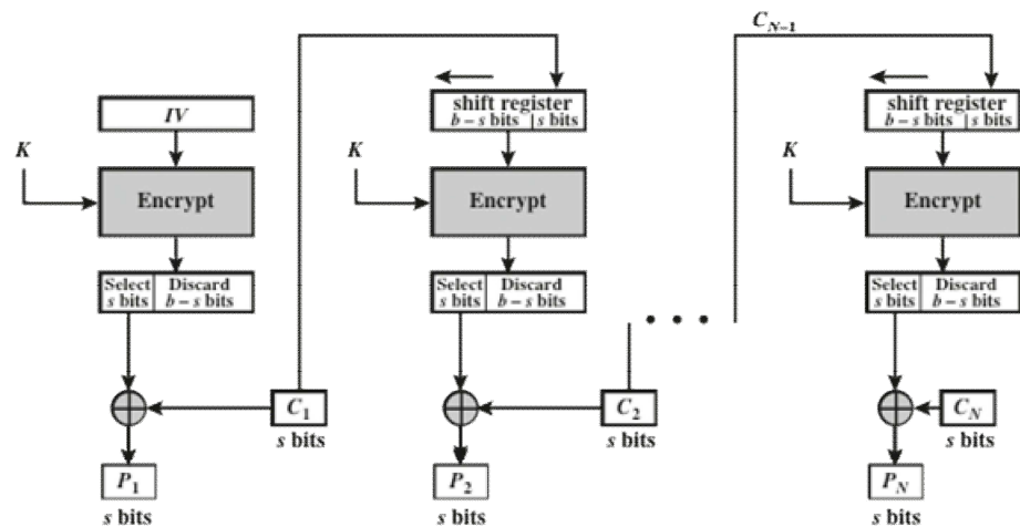
(b) Decryption
