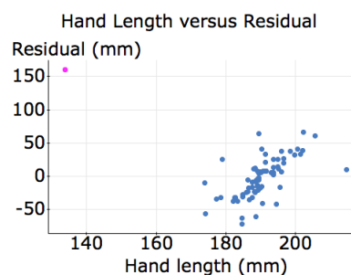
Figure 2.4: Residual plot for hand-height data
