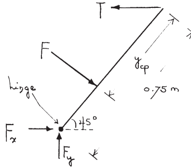
Figure 2.7: Free-Body Diagram
